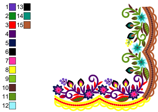
File: corner.jef Stitches: 18732 Size: 175.6x178.6 mm Colors: 14/15 Stops: 14
